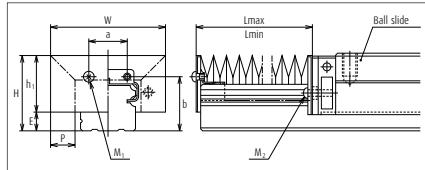
Fig. 17 Dimensions of bellows
