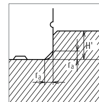
Fig. 5 Shoulder for the rail datum face
