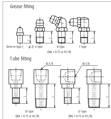
Fig. 7 Grease fitting and tube fitting
