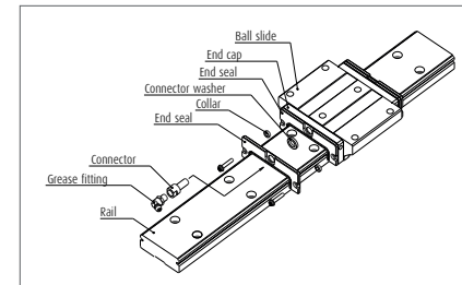
Fig. 10 Double seal
