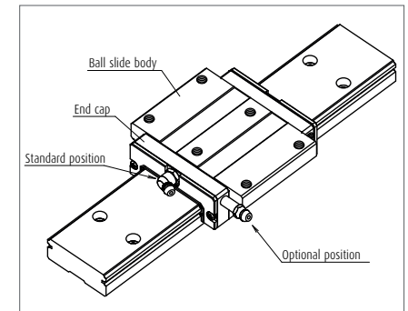
Fig. 8 Mounting position of lubrication accessories
