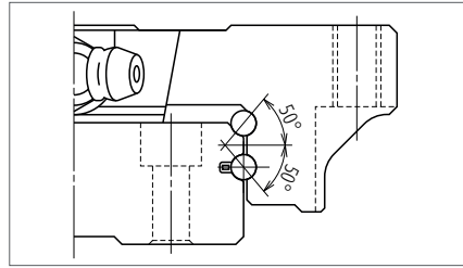
Fig. 1 Balls in contact
