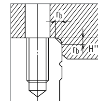
Fig. 6 Shoulder for the ball slide datum face
