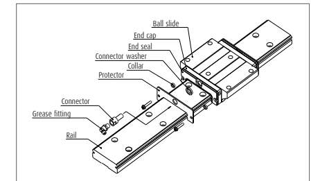
Fig. 11 Protector seal
