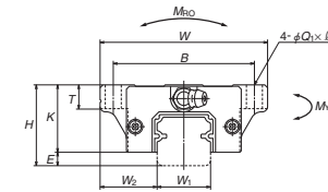
FL and HL types
